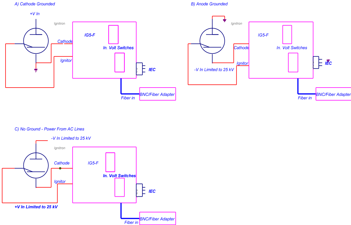
Figure 1 Application scenarios. The metal box should always be grounded.
