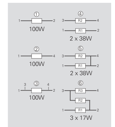
Version 5: ohmic value between contact 2 and 4 = 3mΩ
