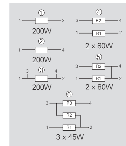
Version 5: ohmic value between contact 2 and 4 = 3mΩ
