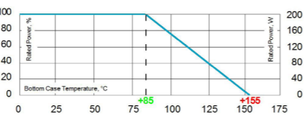
Derating (thermal resist.) HXP-200: 2.86 W/K (0.35 K/W) (for conf. 1, 2 and 3)
