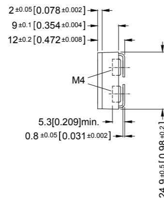
Version 5: ohmic value between contact 2 and 4 = 3mΩ
