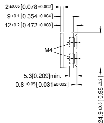
Version 5: ohmic value between contact 2 and 4 = 3mΩ
